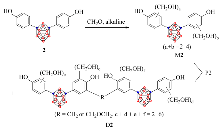
Scheme 2 Synthetic route to m -carborane bisphenol resol phenolic resin (P2)
