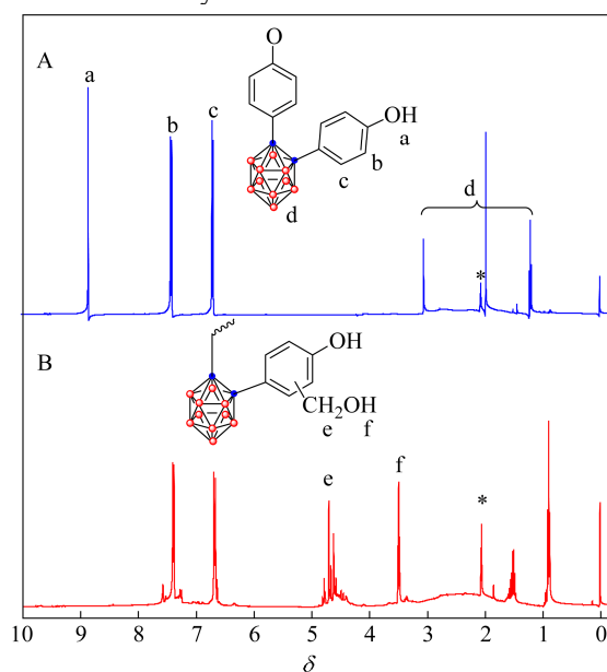
Fig. 4 1 H-NMR spectra of (A) o -carborane bisphenol ( 1 ), and (B) o -carborane bisphenol resol phenolic resin ( P1 , Table 1, No. 5) in acetone- d 6 (The solvent peaks are marked with asterisks.)
