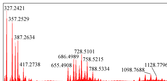
Fig. 1 High resolution mass spectrum of P1 (Table 1, No. 5)
